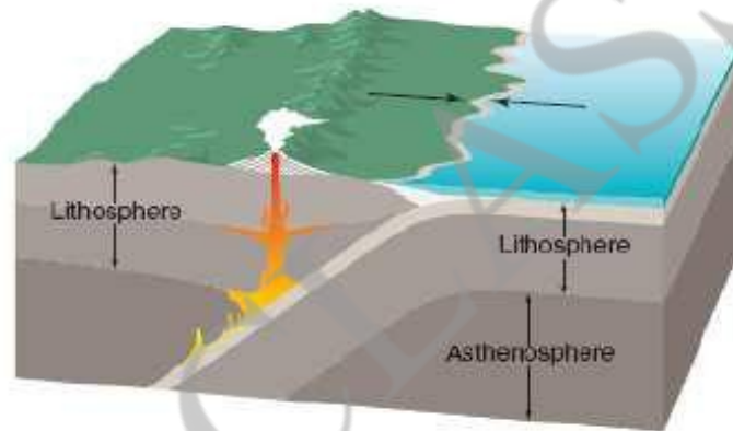
FIG: 6 A convergent plate boundary where an oceanic plate subducts under a continental plate
